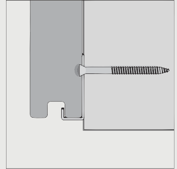
C-Clip
