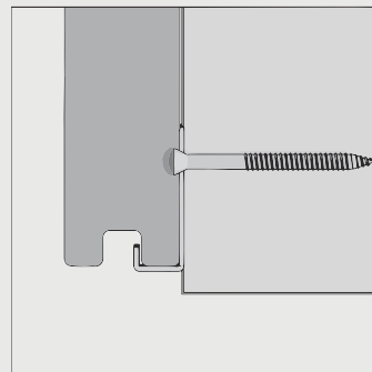
C-Clip
